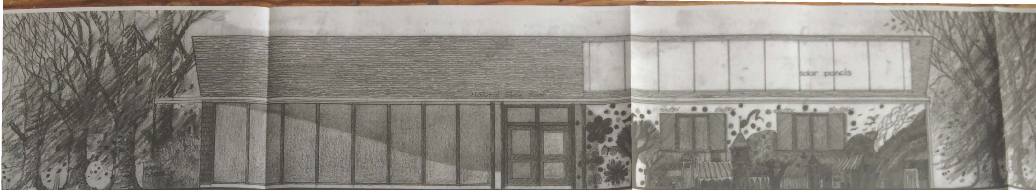
PROPOSED ELEVATION TO THE NORTH EAST, scale: 1:50
